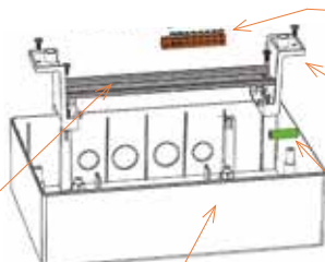
ЗНІМНА DIN-РЕЙКА Easy installation cause of fuse rail which is together with rail carrier
